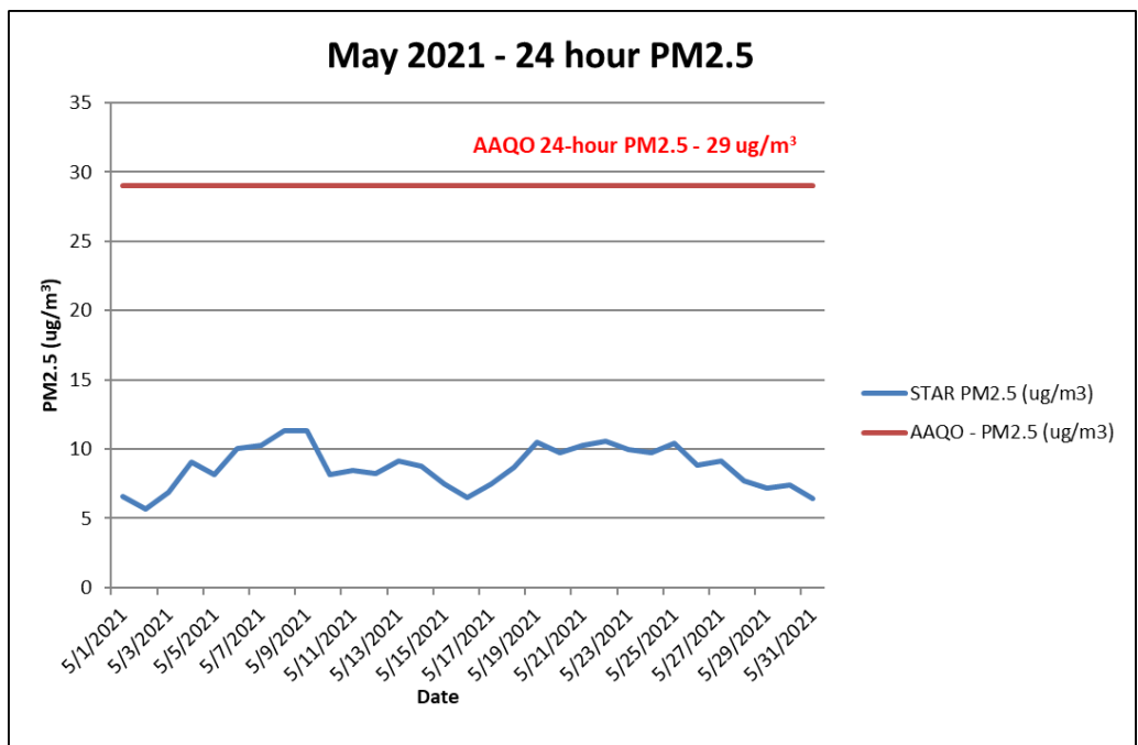
Figure 4: 24-hour concentrations of PM 2.5 at STAR
