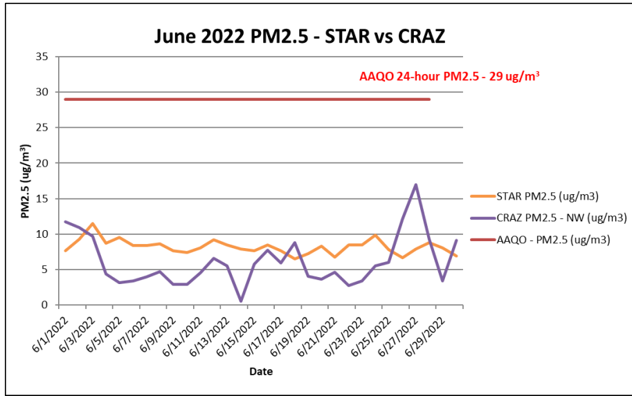
Figure 5: CRAZ and STAR Comparison for PM 2.5
