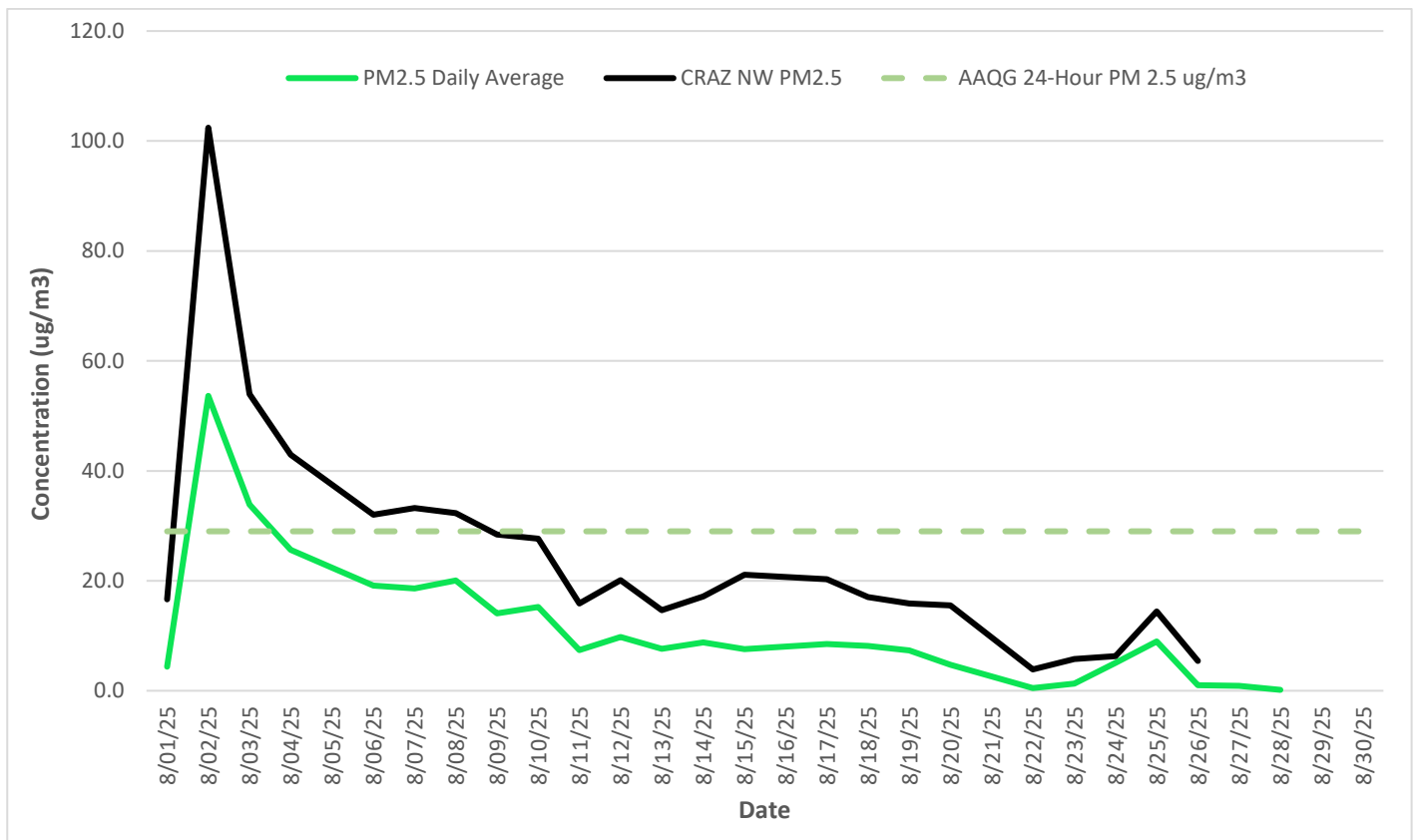
Figure 4. STAR PIT – September 2025 – PM 2.5 Daily Particulate Monitoring Results
