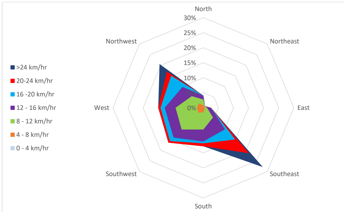
Figure 5. STAR PIT Trailer – September 2025 - Wind Rose
