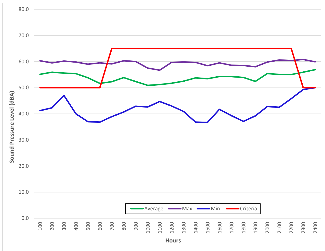
Figure 2. STAR PIT – September 2025 – Hourly Sound Monitoring Summary
