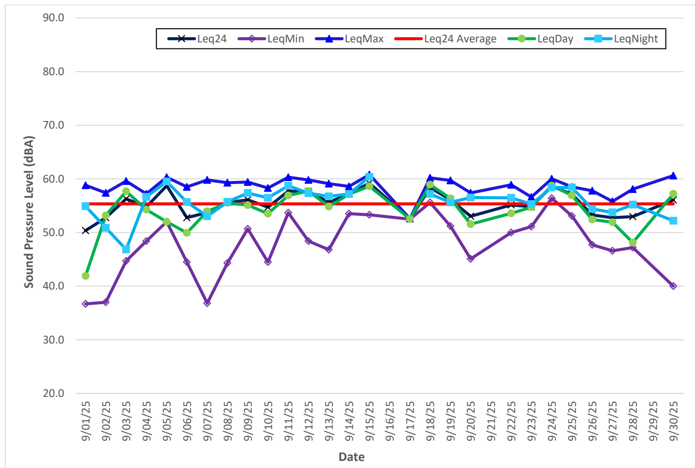
Figure 1. STAR PIT – September 2025 – Daily Sound Monitoring Results
