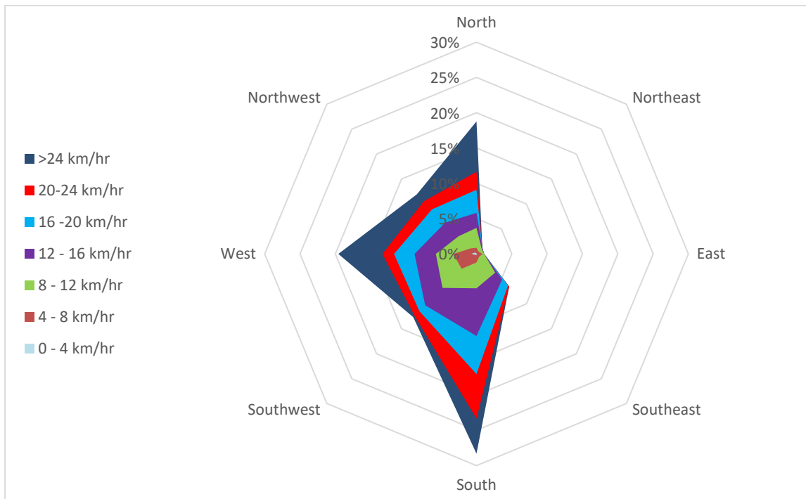
Figure 6. STAR PIT Office – September 2025 - Wind Rose
